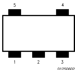
5-Lead Small Outline Package (M5)
